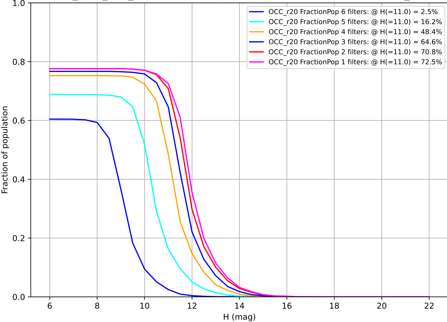
four_cycle_v3.5_10yrs: Fraction of population with colors in X filters OCC_r20
