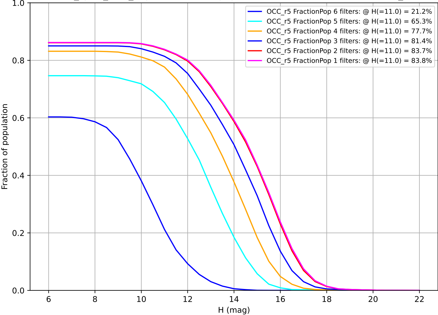
four_cycle_v3.5_10yrs: Fraction of population with colors in X filters OCC_r5
