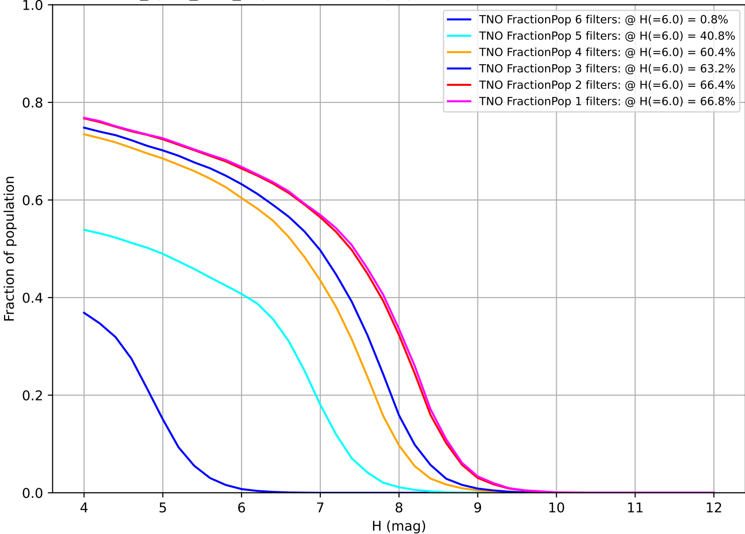
four_cycle_v3.5_10yrs: Fraction of population with colors in X filters TNO
