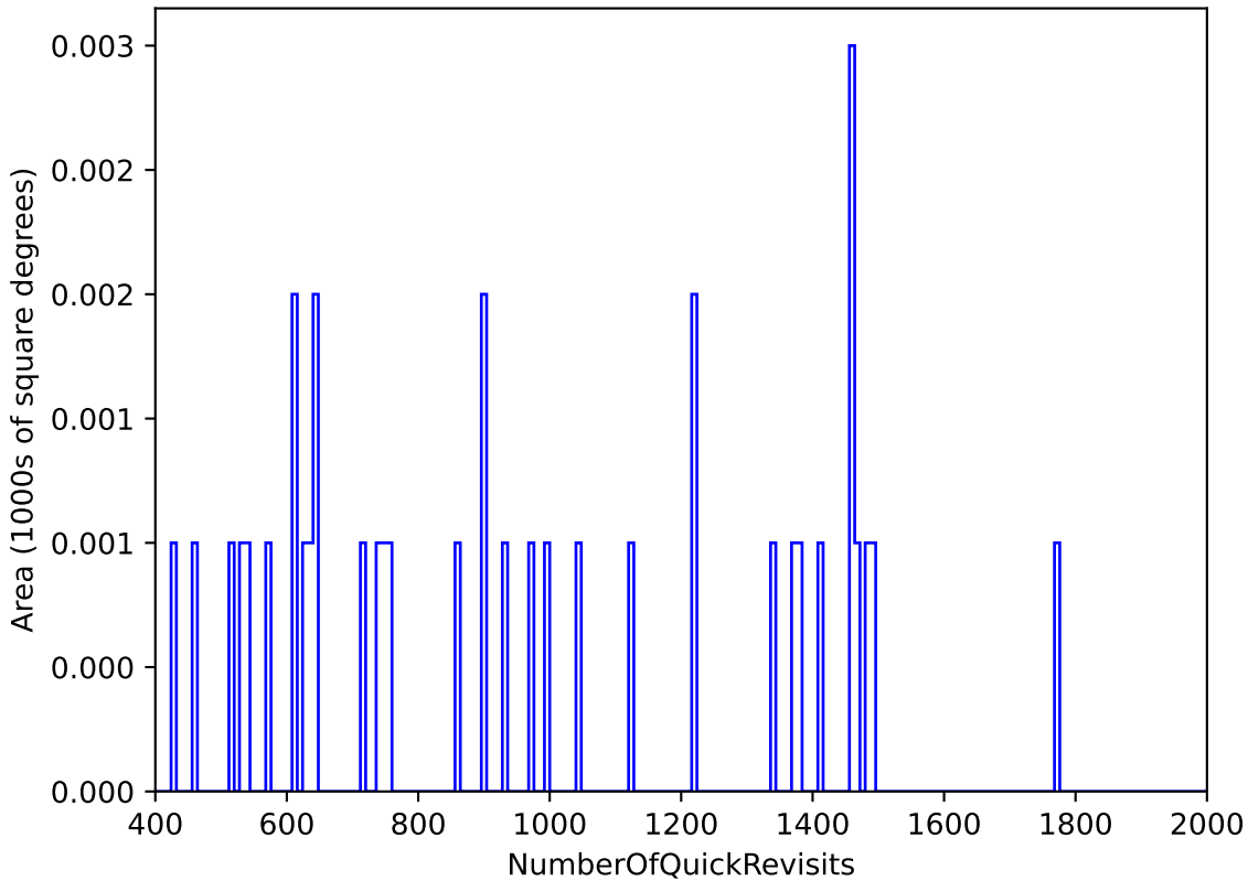
four_cycle_v3.6_10yrs : NumberOfQuickRevisits
