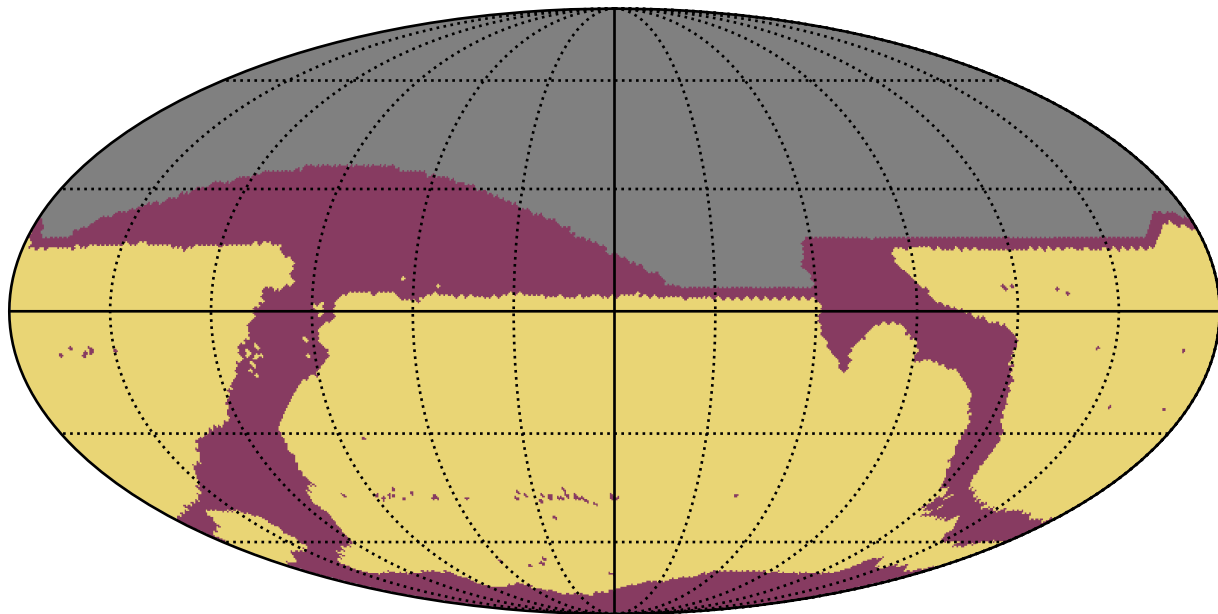
four_cycle_v3.6_10yrs : RapidRevisits
