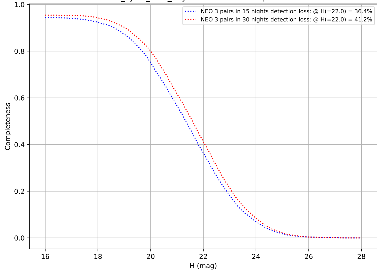
four_cycle_v3.6_10yrs: DifferentialCompleteness
