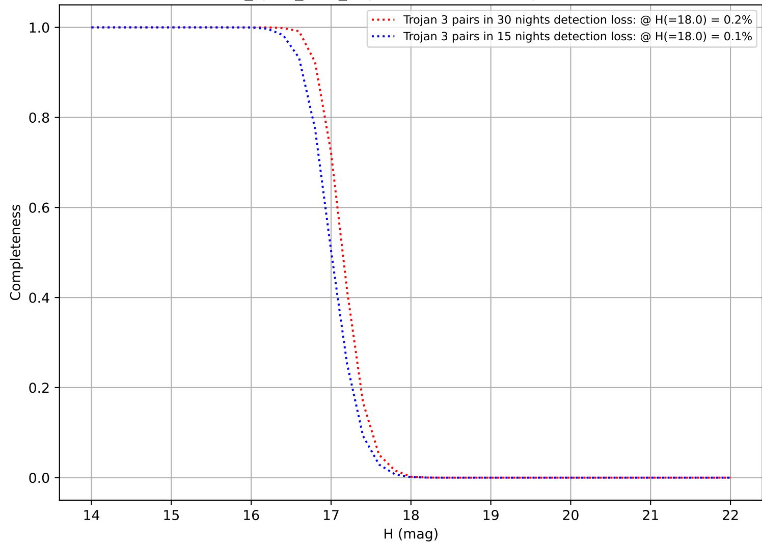
four_cycle_v3.6_10yrs: DifferentialCompleteness
