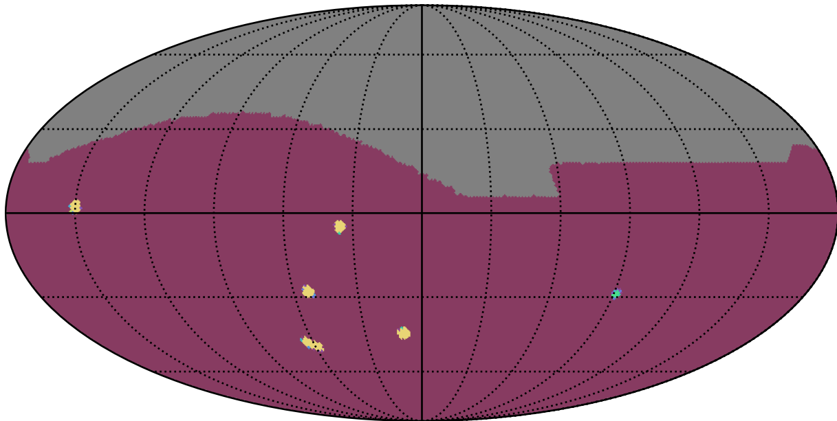
four_cycle_v4.0_10yrs : NumberOfQuickRevisits
