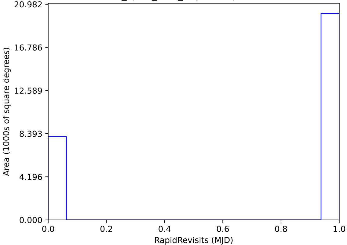
four_cycle_v4.0_10yrs : RapidRevisits
