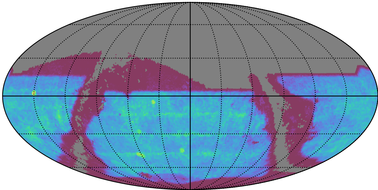
four_cycle_v4.0_10yrs : SNSLMetric
