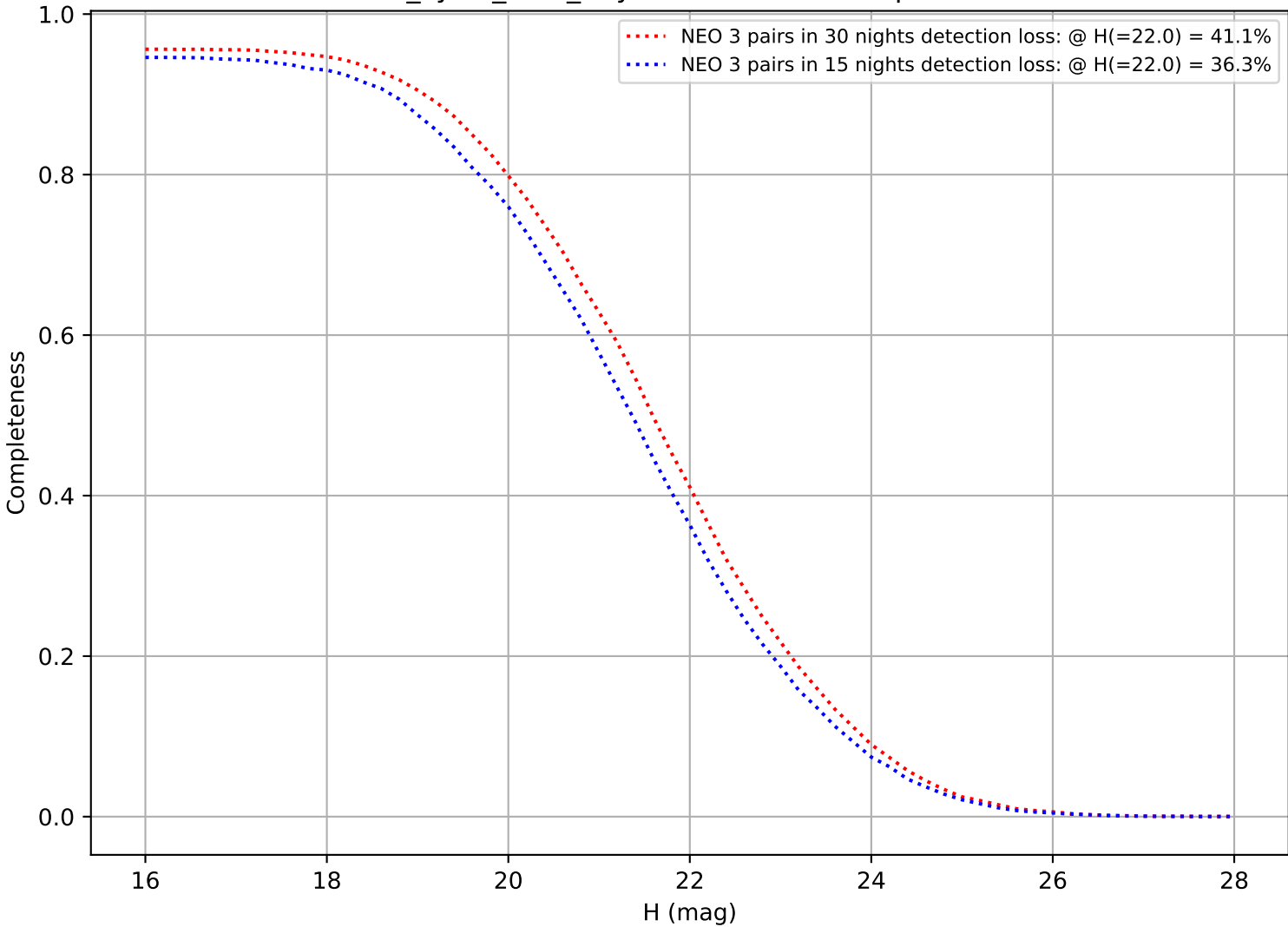
four_cycle_v4.0_10yrs: DifferentialCompleteness
