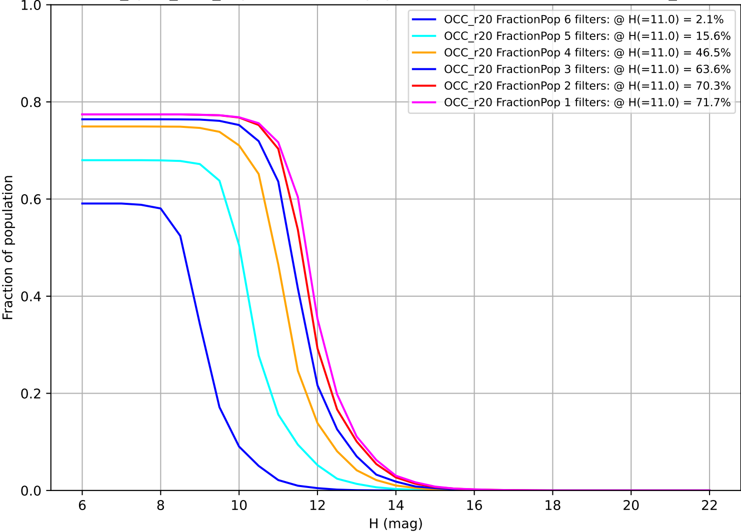
four_cycle_v4.0_10yrs: Fraction of population with colors in X filters OCC_r20
