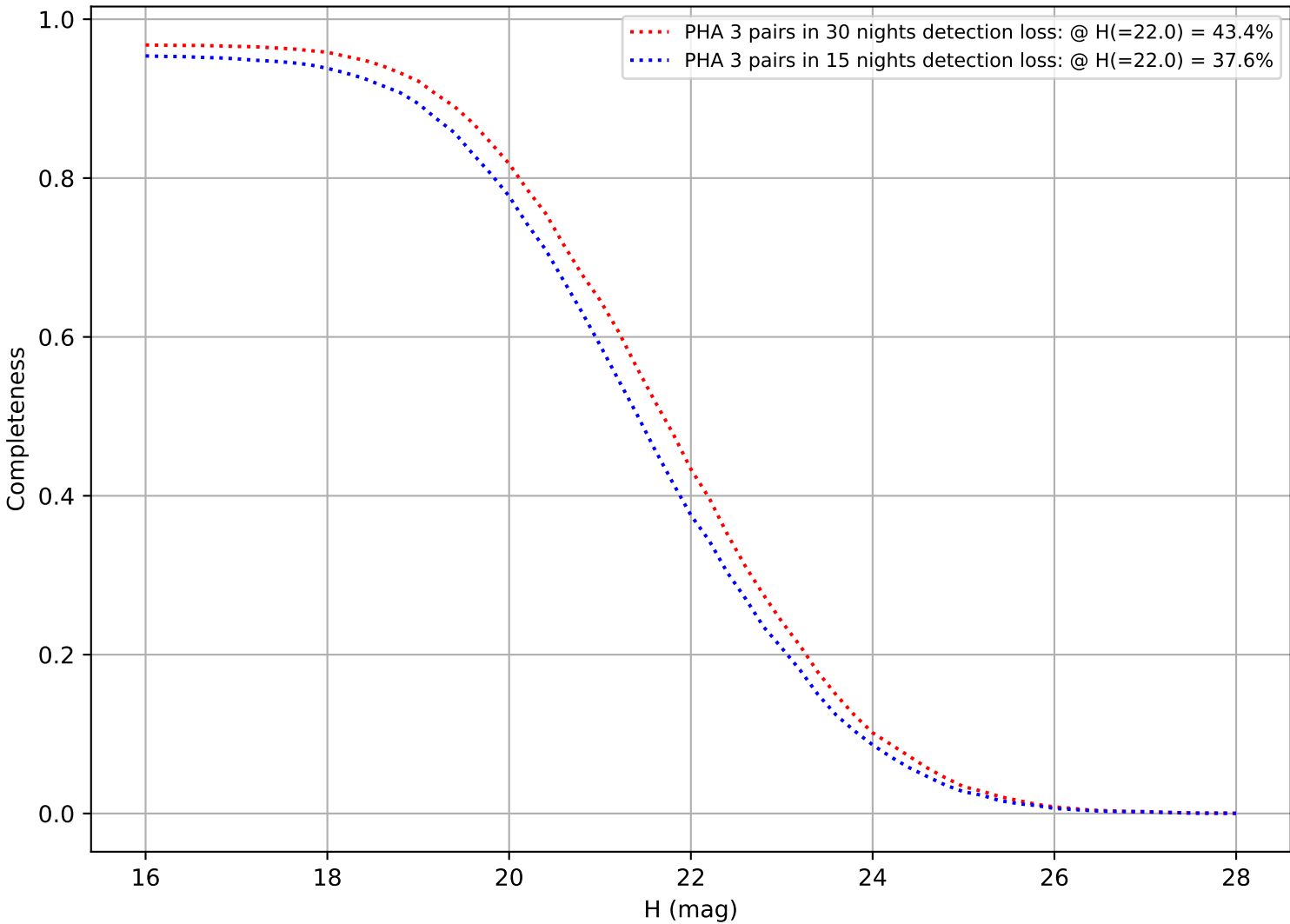
four_cycle_v4.0_10yrs: DifferentialCompleteness
