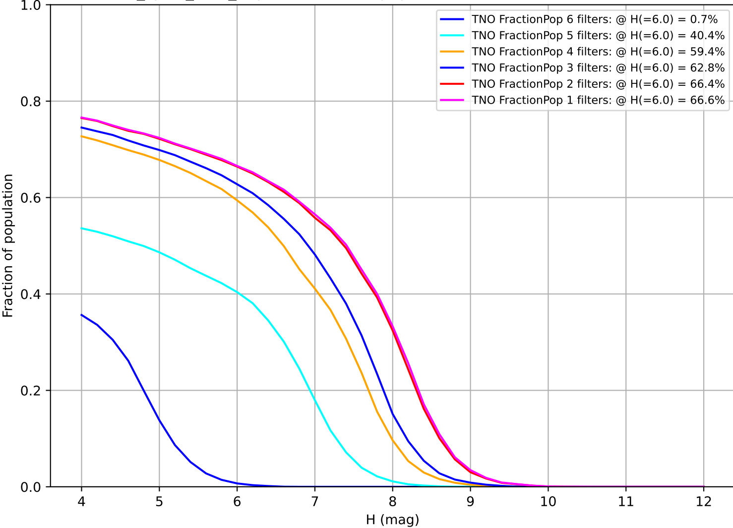
four_cycle_v4.0_10yrs: Fraction of population with colors in X filters TNO
