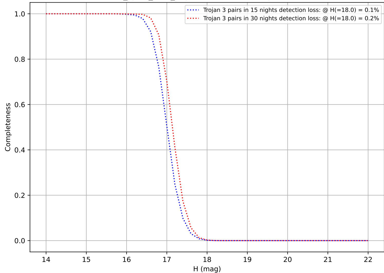
four_cycle_v4.0_10yrs: DifferentialCompleteness
