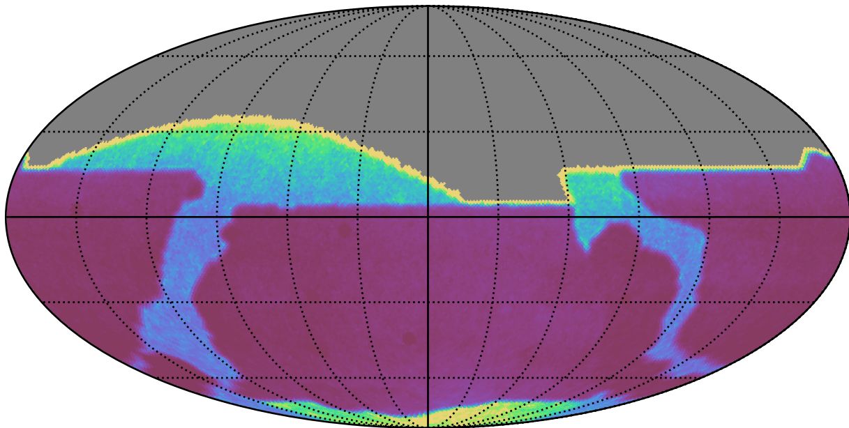
no_too_v3.6_10yrs : properMotion
