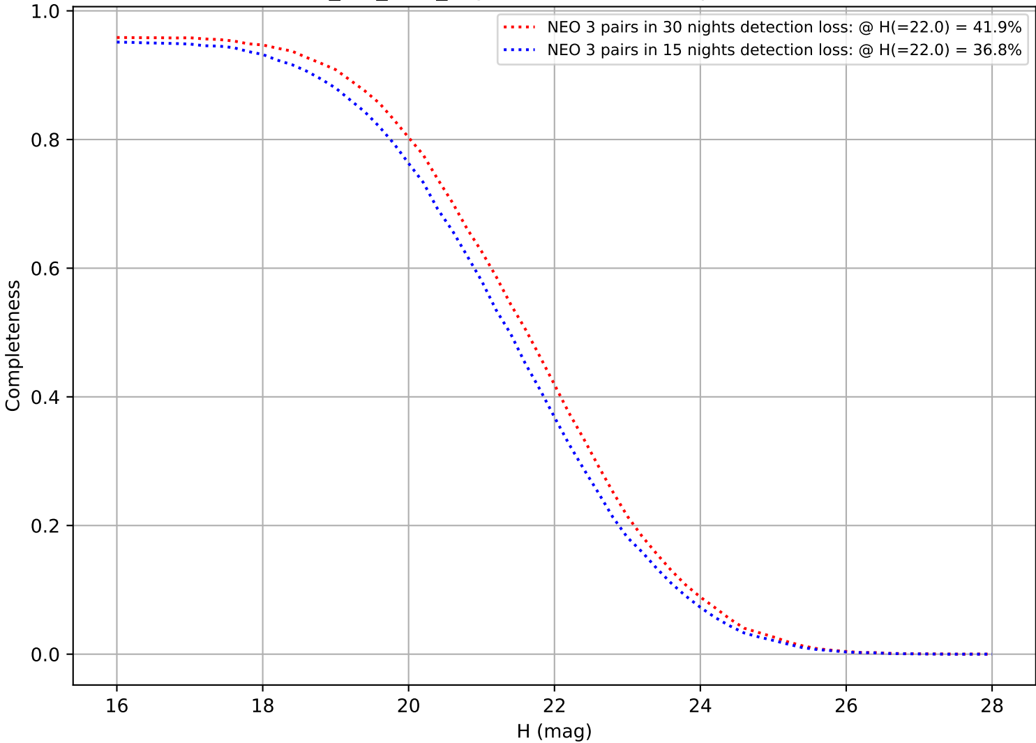
no_too_v3.6_10yrs: DifferentialCompleteness
