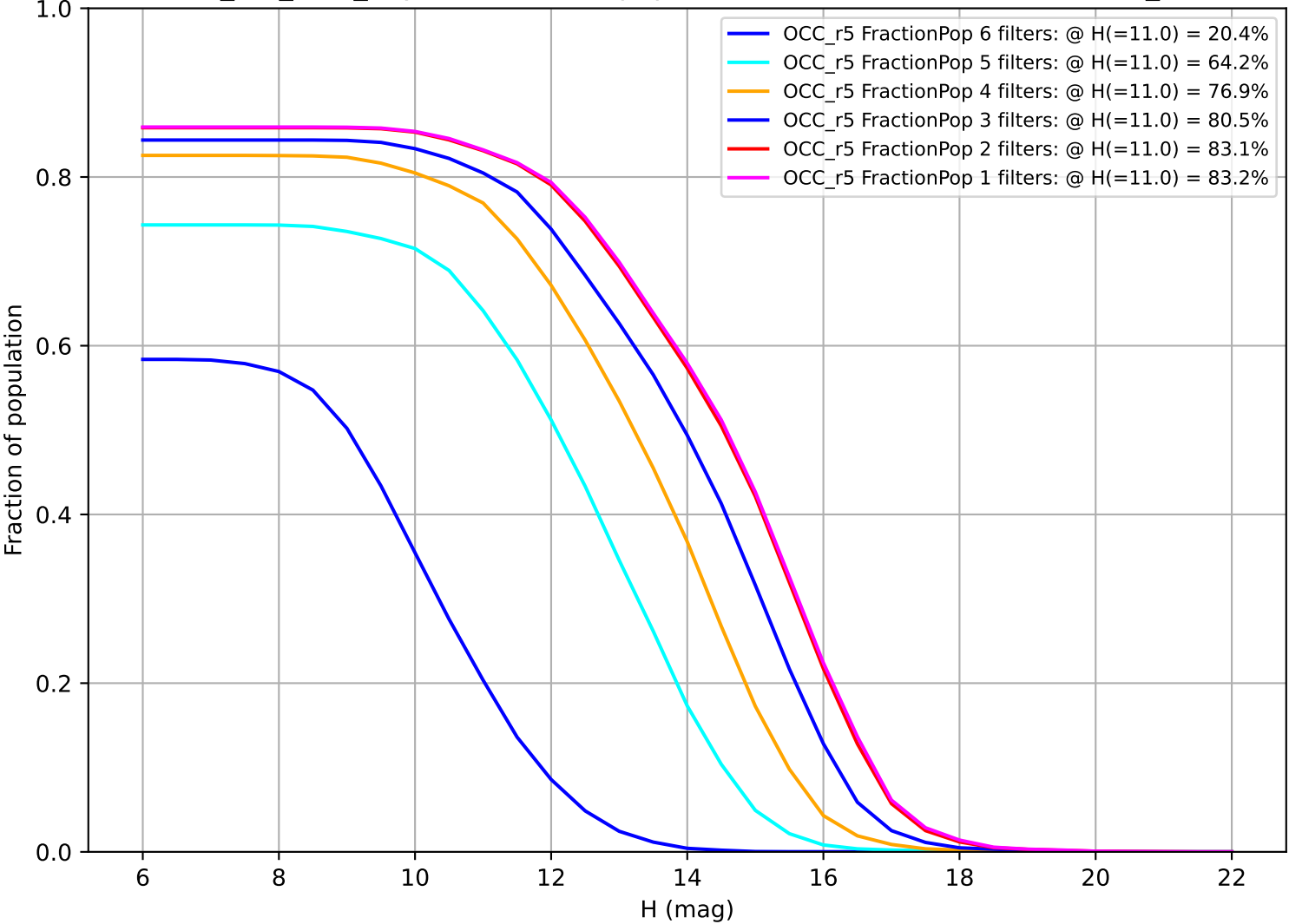
no_too_v3.6_10yrs: Fraction of population with colors in X filters OCC_r5
