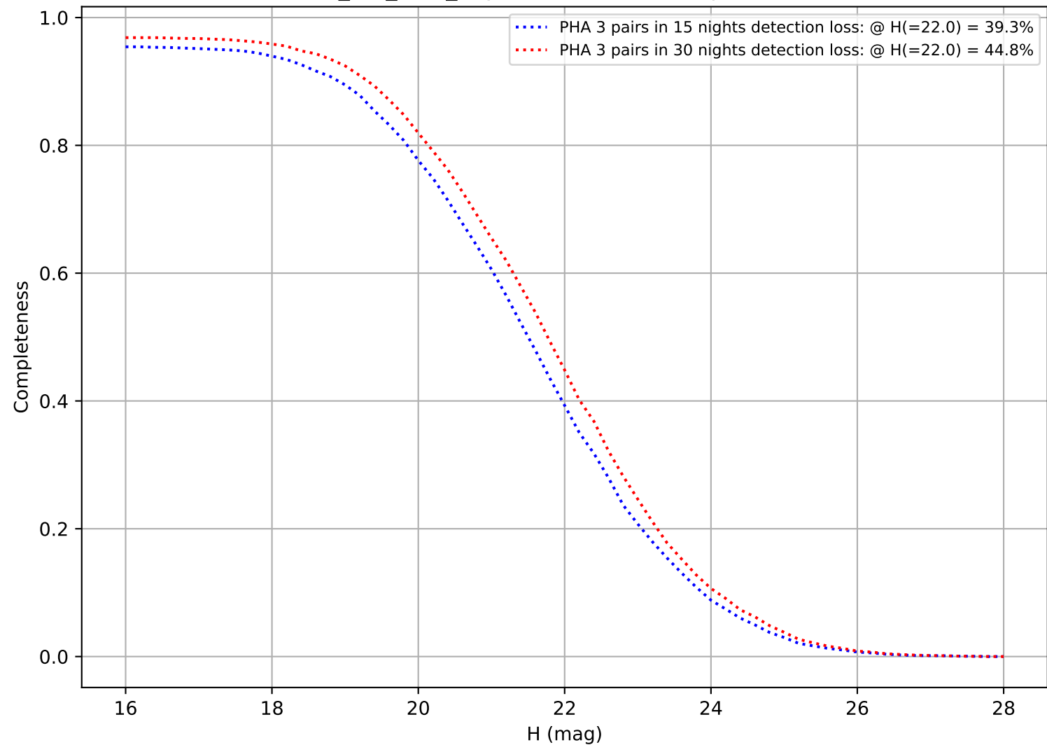
no_too_v3.6_10yrs: DifferentialCompleteness
