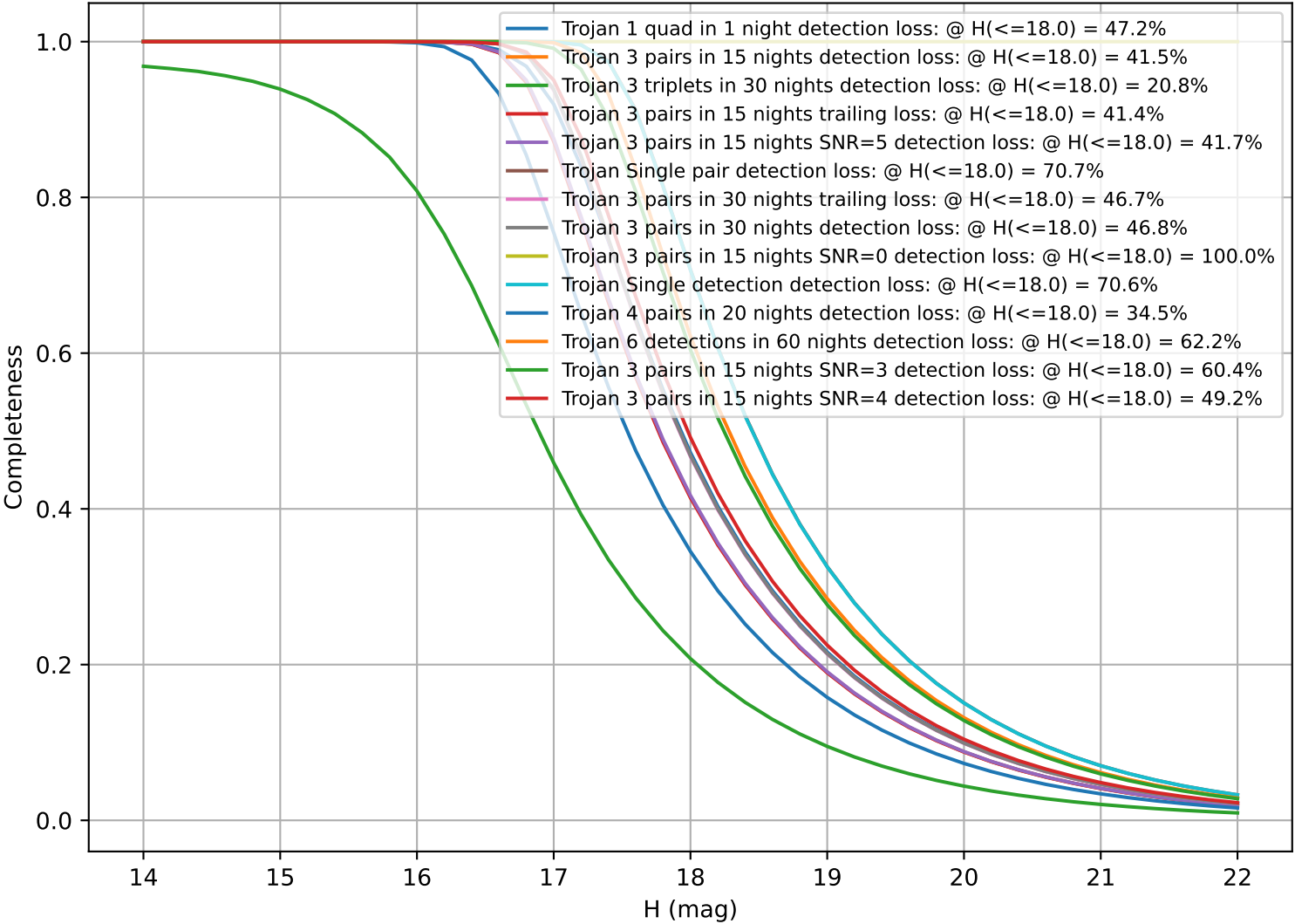
no_too_v3.6_10yrs: CumulativeCompleteness
