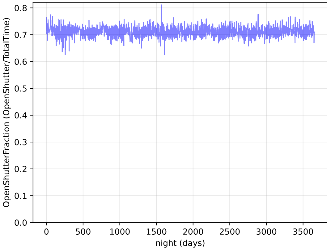
no_too_v4.0_10yrs : OpenShutterFraction
