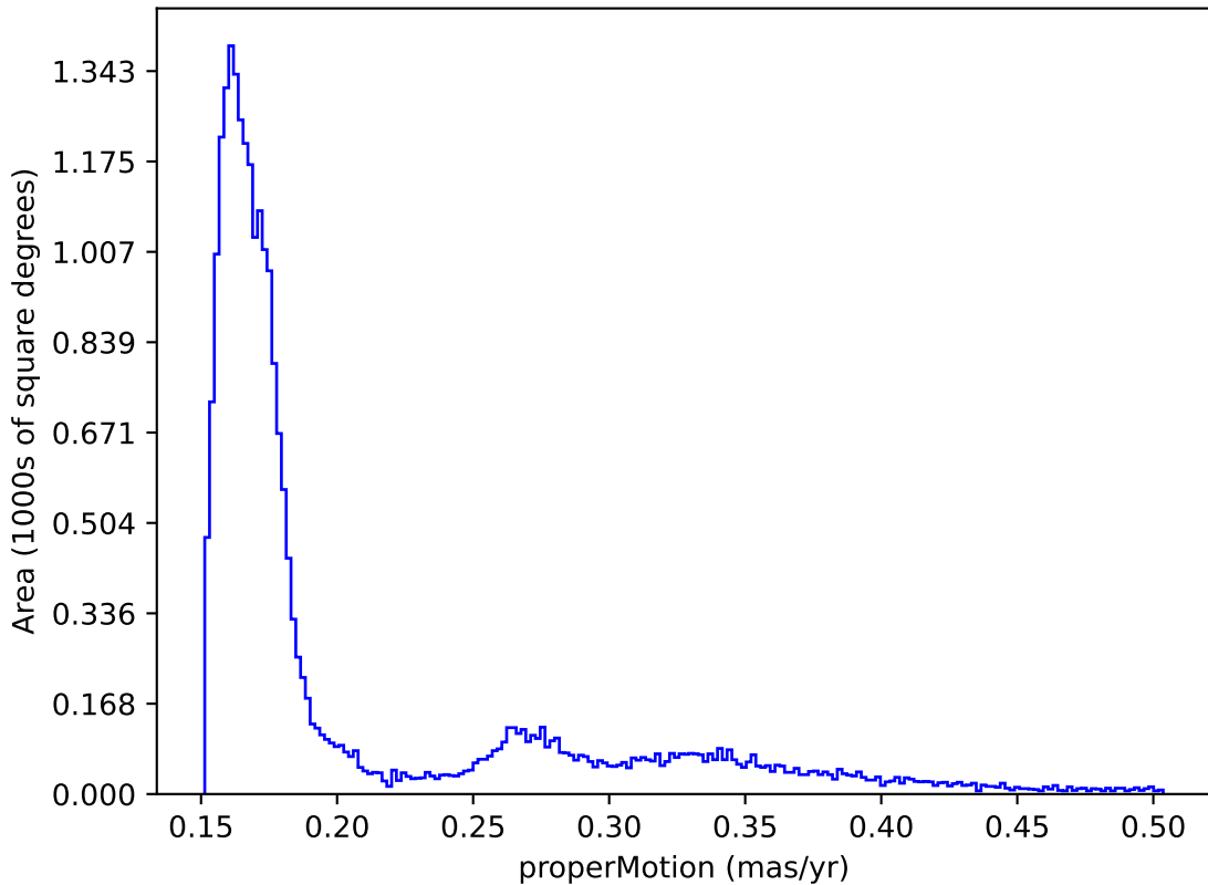
no_too_v4.0_10yrs : properMotion
