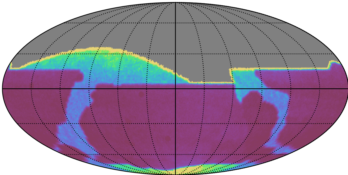
no_too_v4.0_10yrs : properMotion
