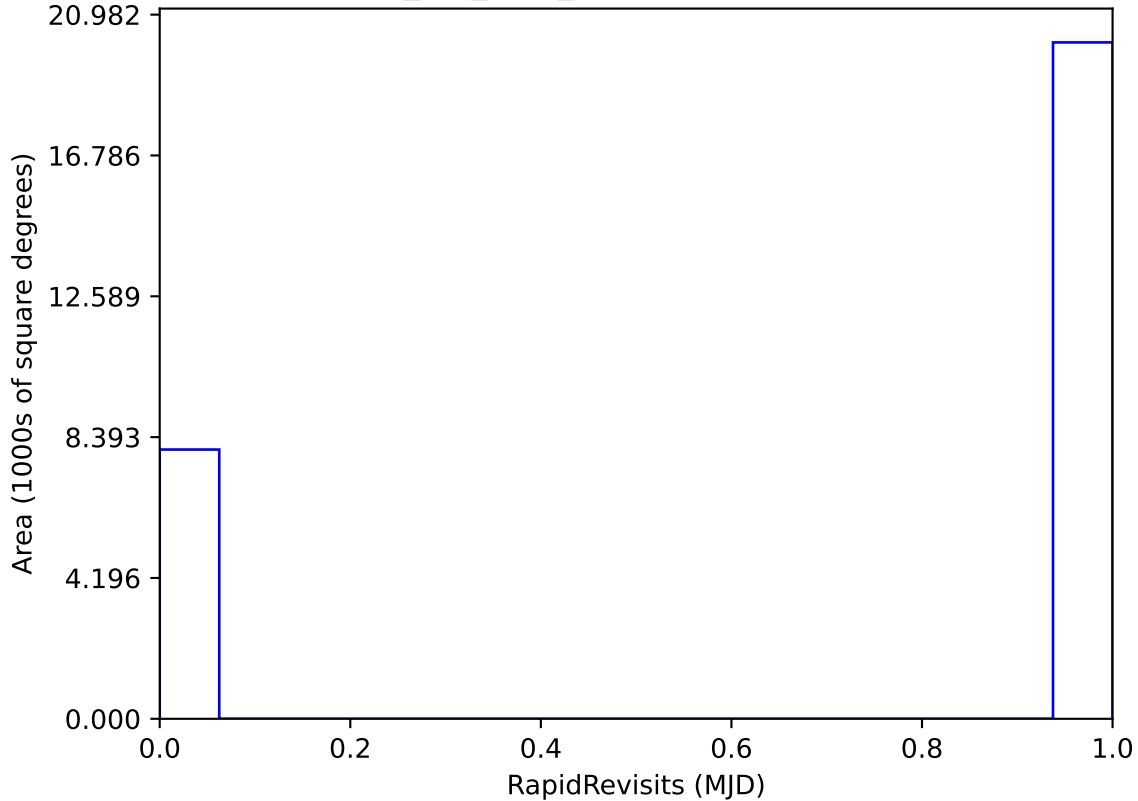
no_too_v4.0_10yrs : RapidRevisits
