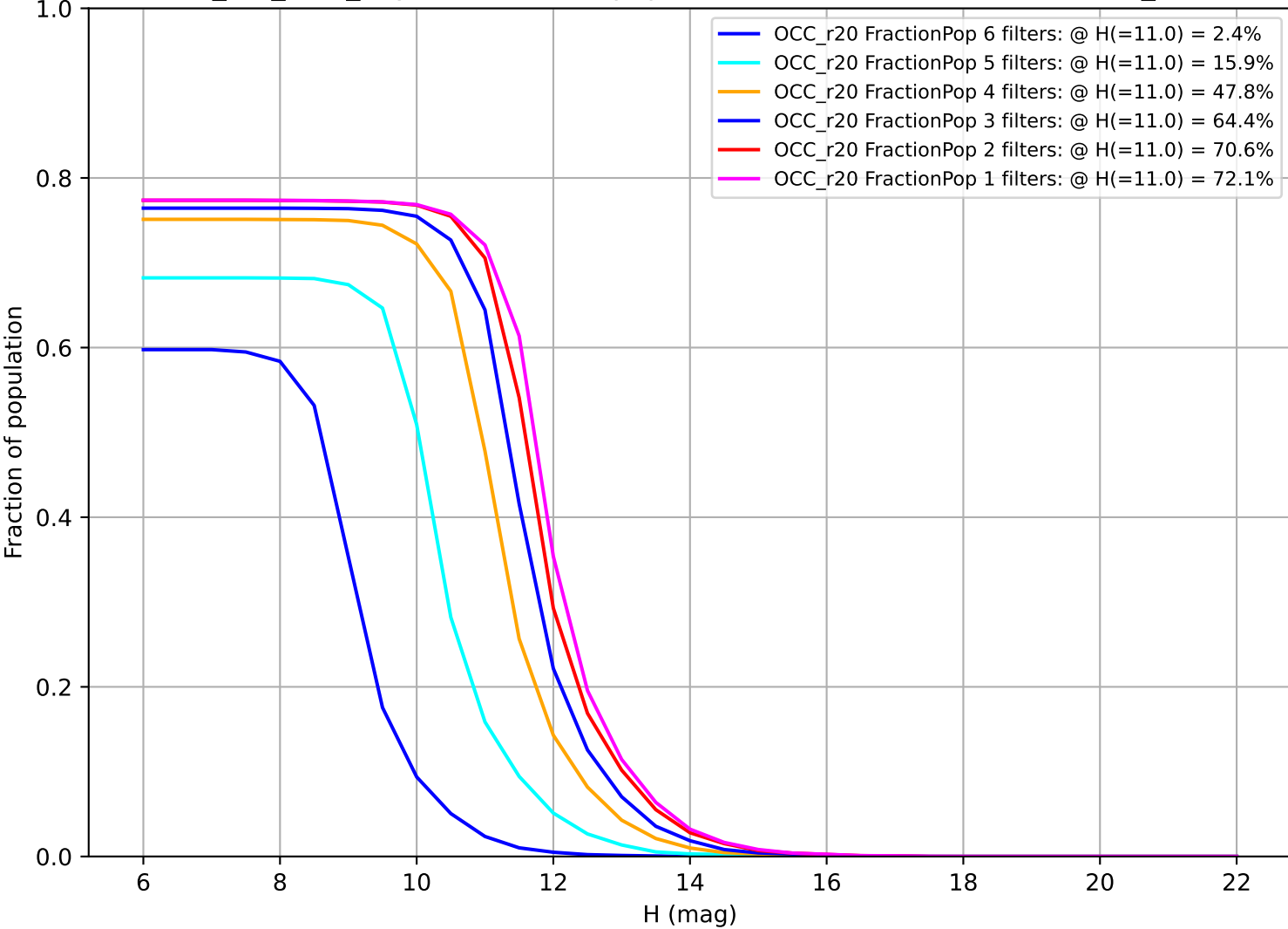
no_too_v4.0_10yrs: Fraction of population with colors in X filters OCC_r20
