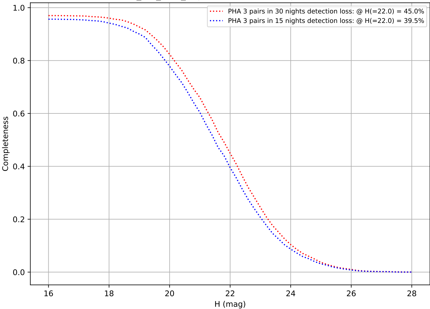
no_too_v4.0_10yrs: DifferentialCompleteness
