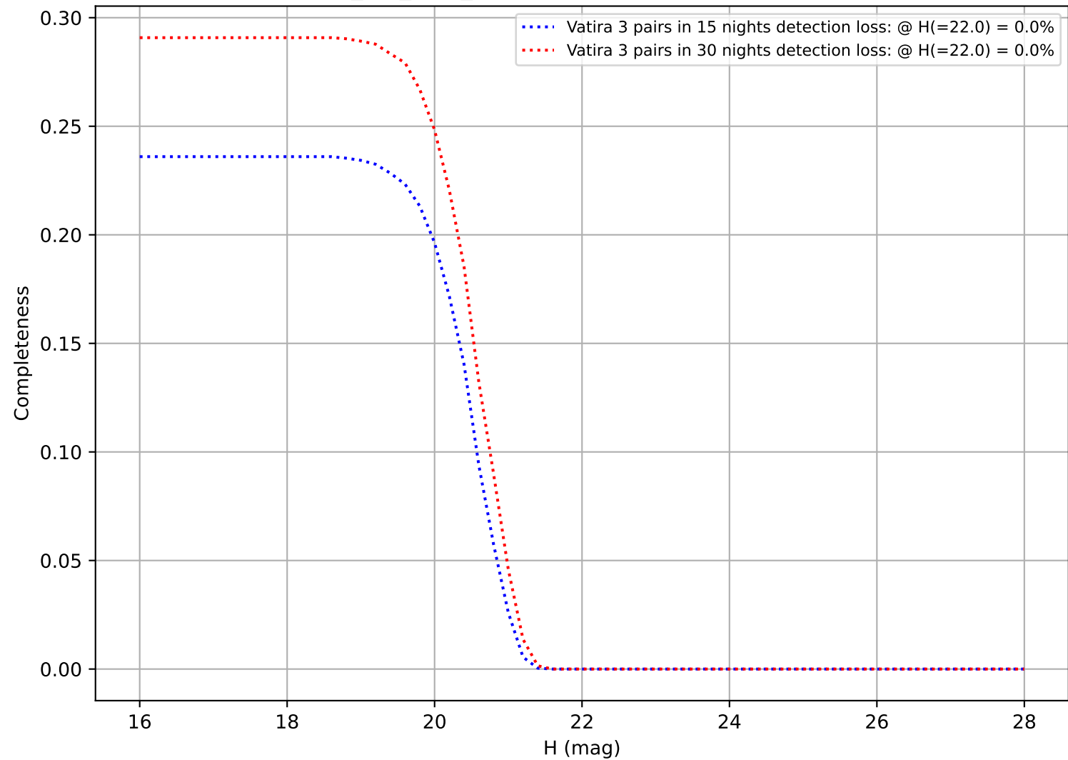
no_too_v4.0_10yrs: DifferentialCompleteness
