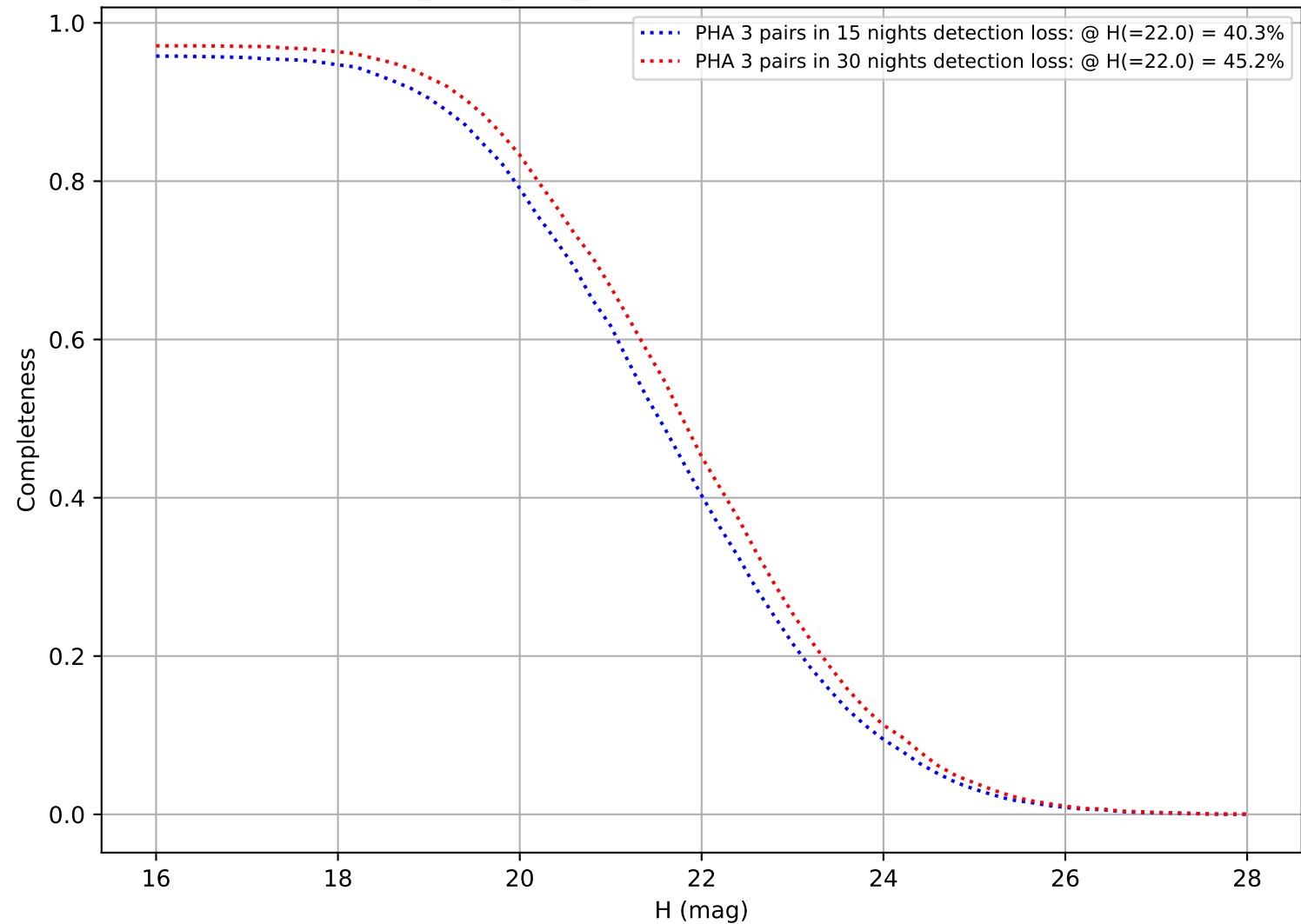
one_snap_v3.6_10yrs: DifferentialCompleteness
