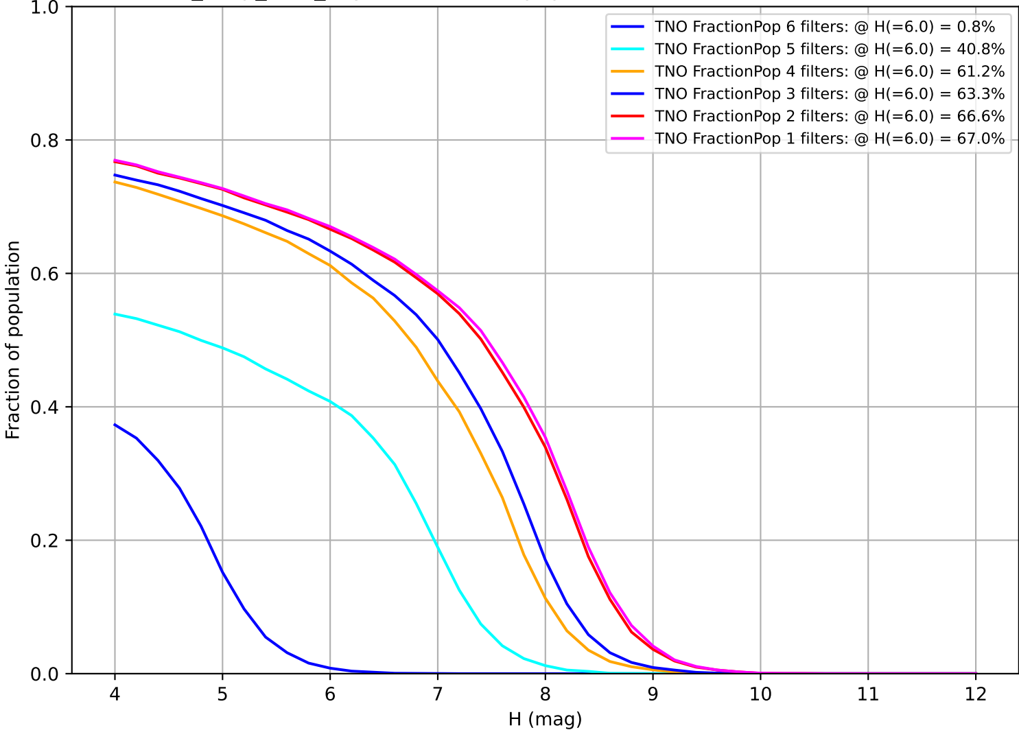
one_snap_v3.6_10yrs: Fraction of population with colors in X filters TNO
