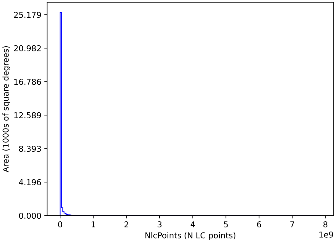
one_snap_v4.0_10yrs : NlcPoints
