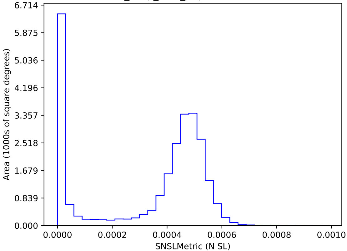
one_snap_v4.0_10yrs : SNSLMetric
