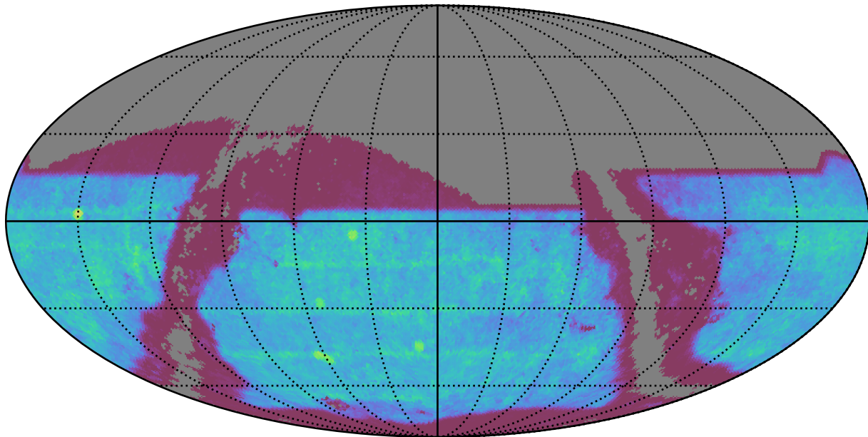
one_snap_v4.0_10yrs : SNSLMetric
