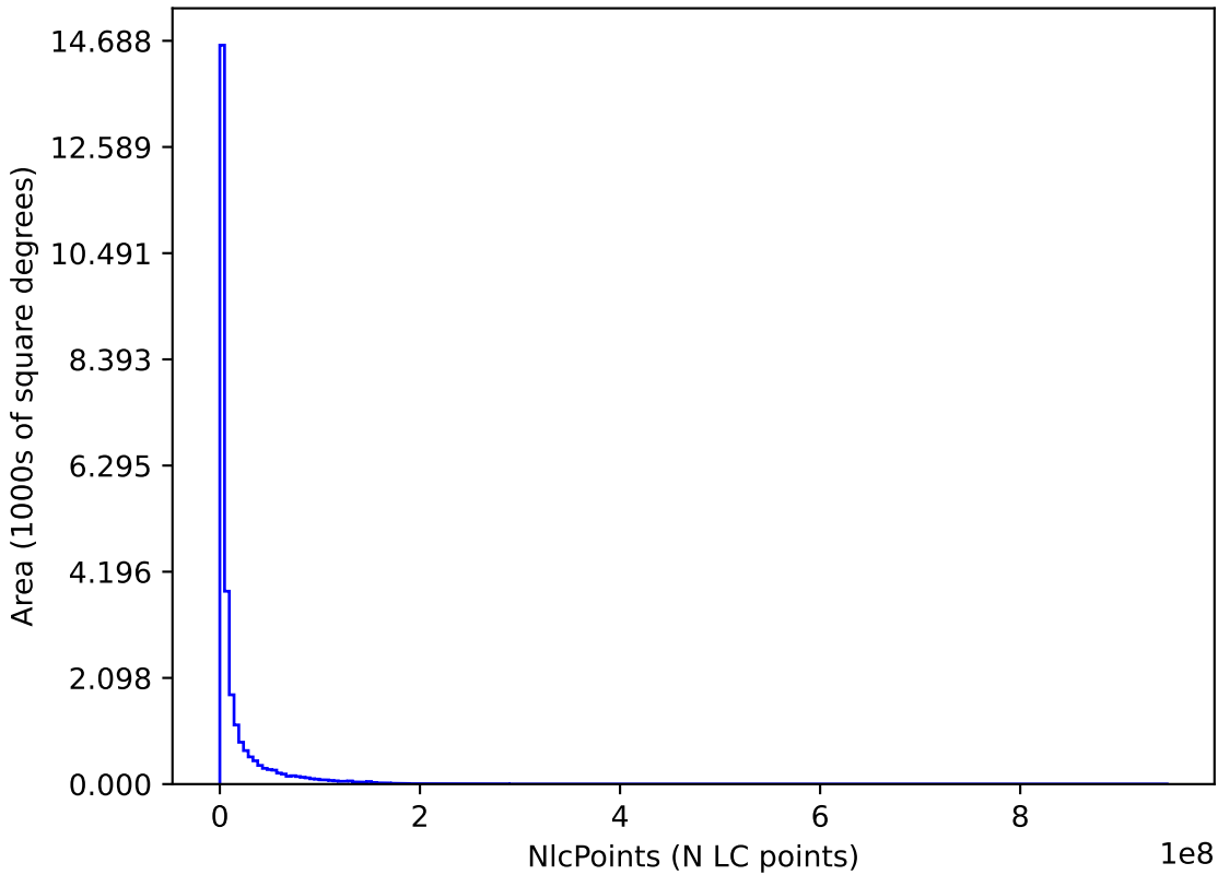
retro_baseline_v2.0_10yrs : NlcPoints
