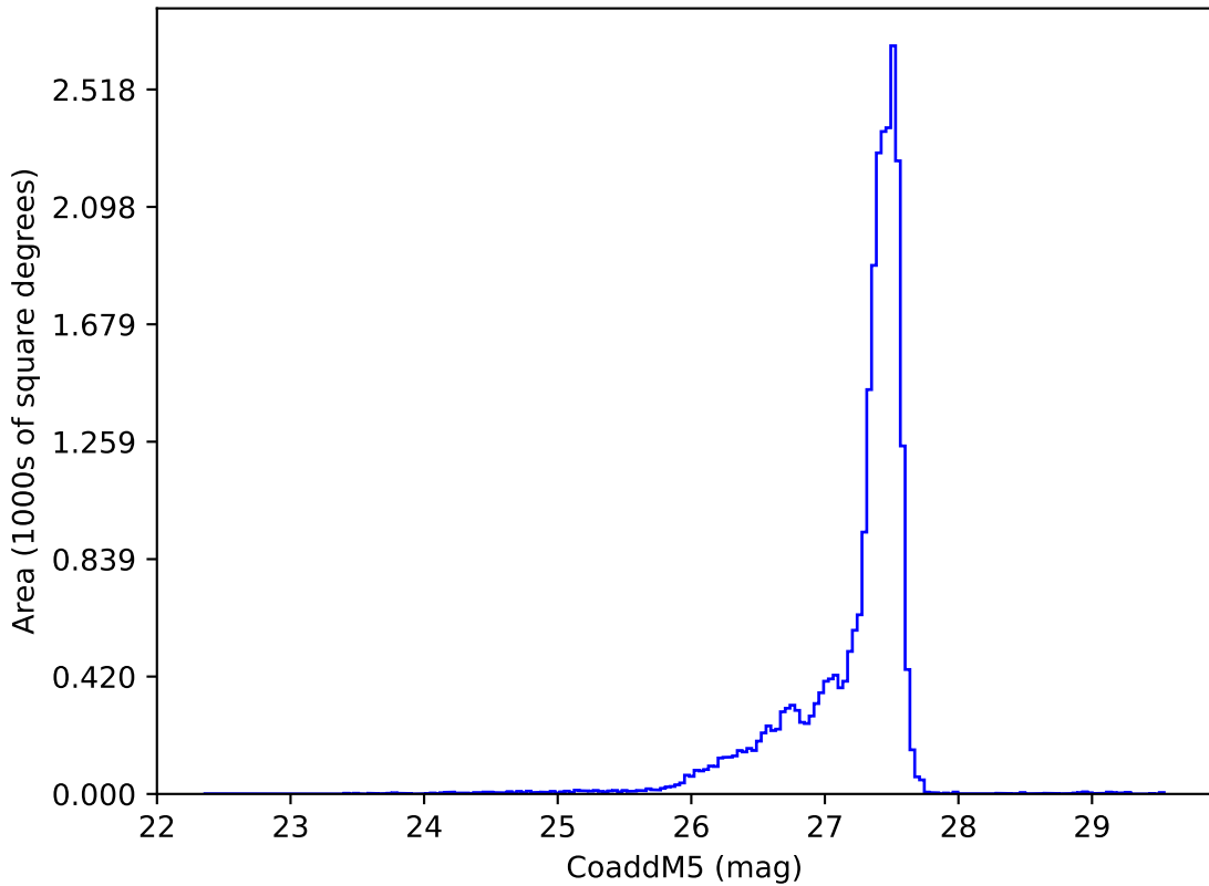
telescope_jerk_v3.5_10yrs : CoaddM5
