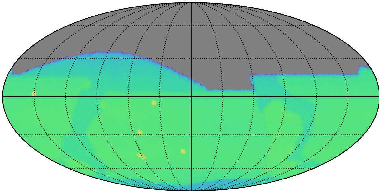
telescope_jerk_v3.5_10yrs : CoaddM5
