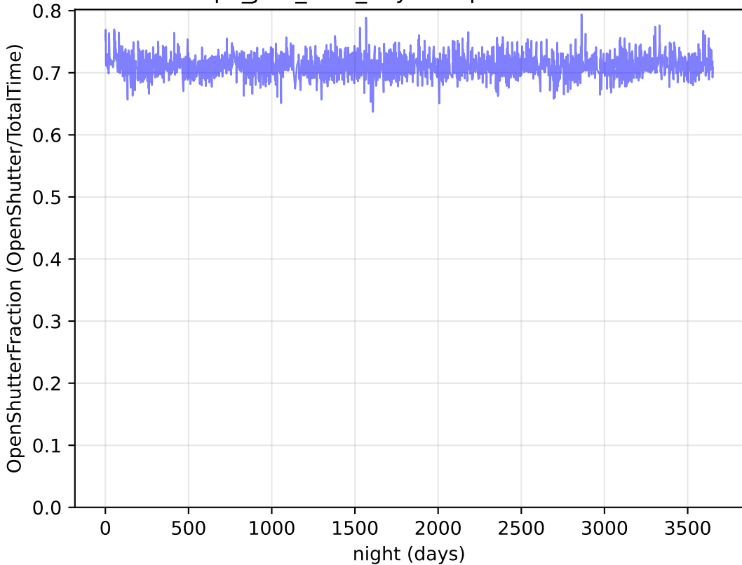
telescope_jerk_v3.5_10yrs : OpenShutterFraction
