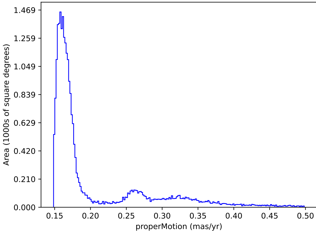
telescope_jerk_v3.5_10yrs : properMotion
