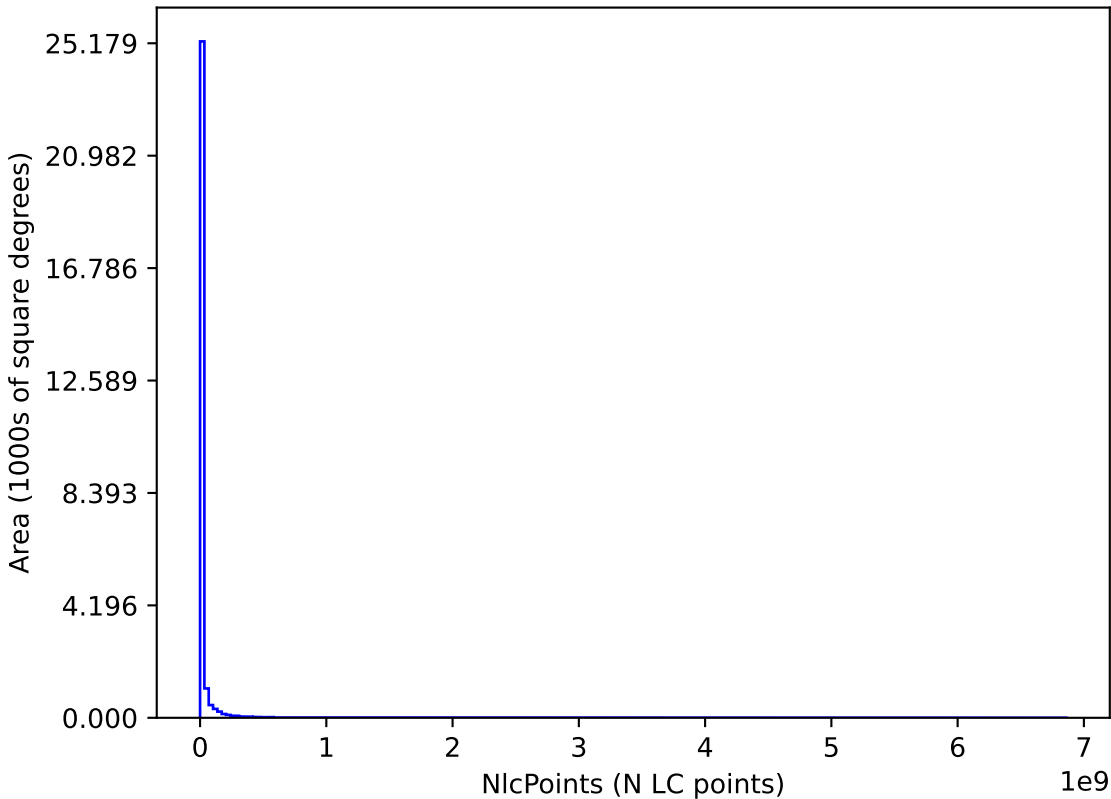
telescope_jerk_v3.5_10yrs : NlcPoints
