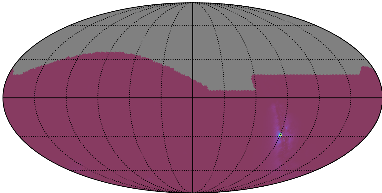
telescope_jerk_v3.5_10yrs : NlcPoints
