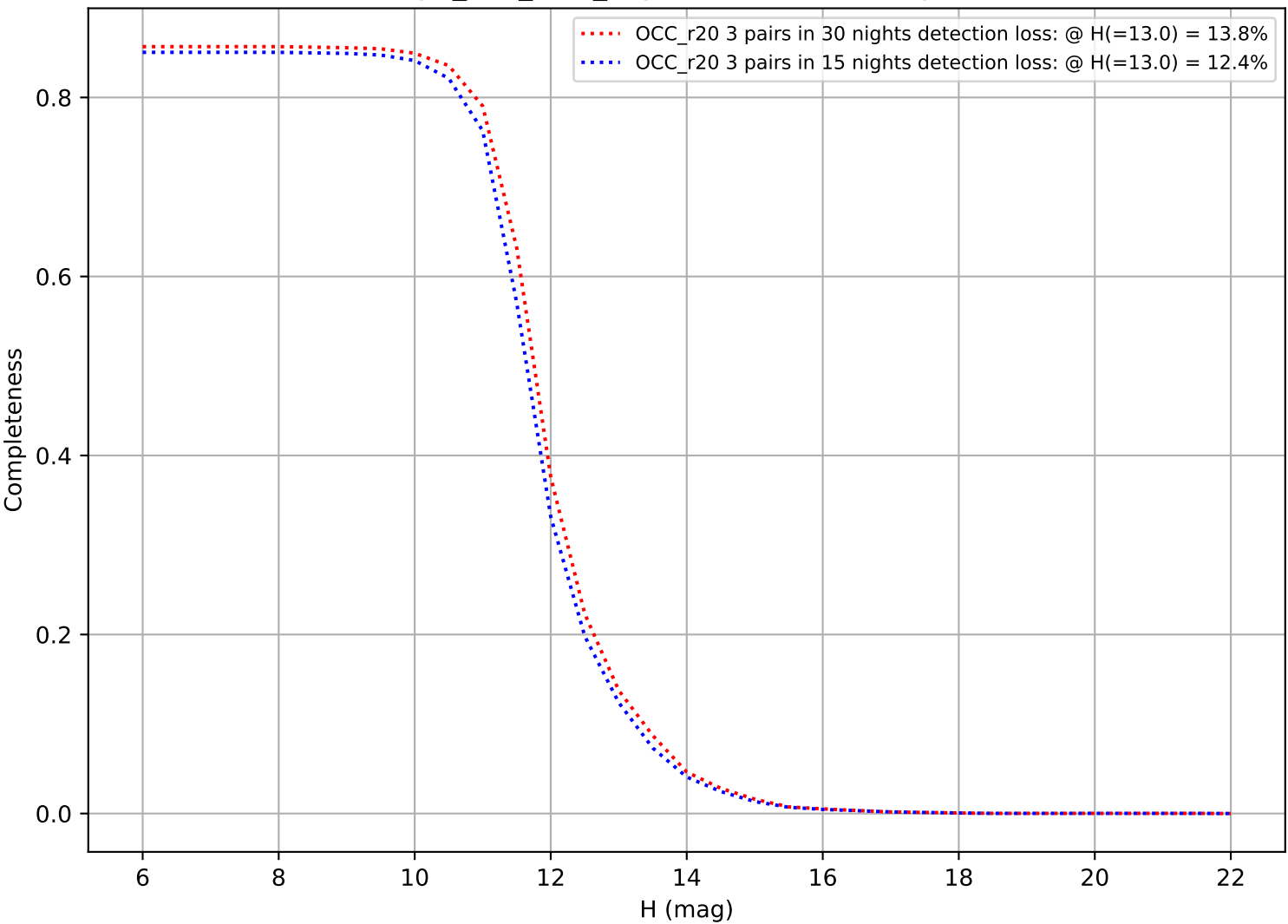
telescope_jerk_v3.5_10yrs: DifferentialCompleteness
