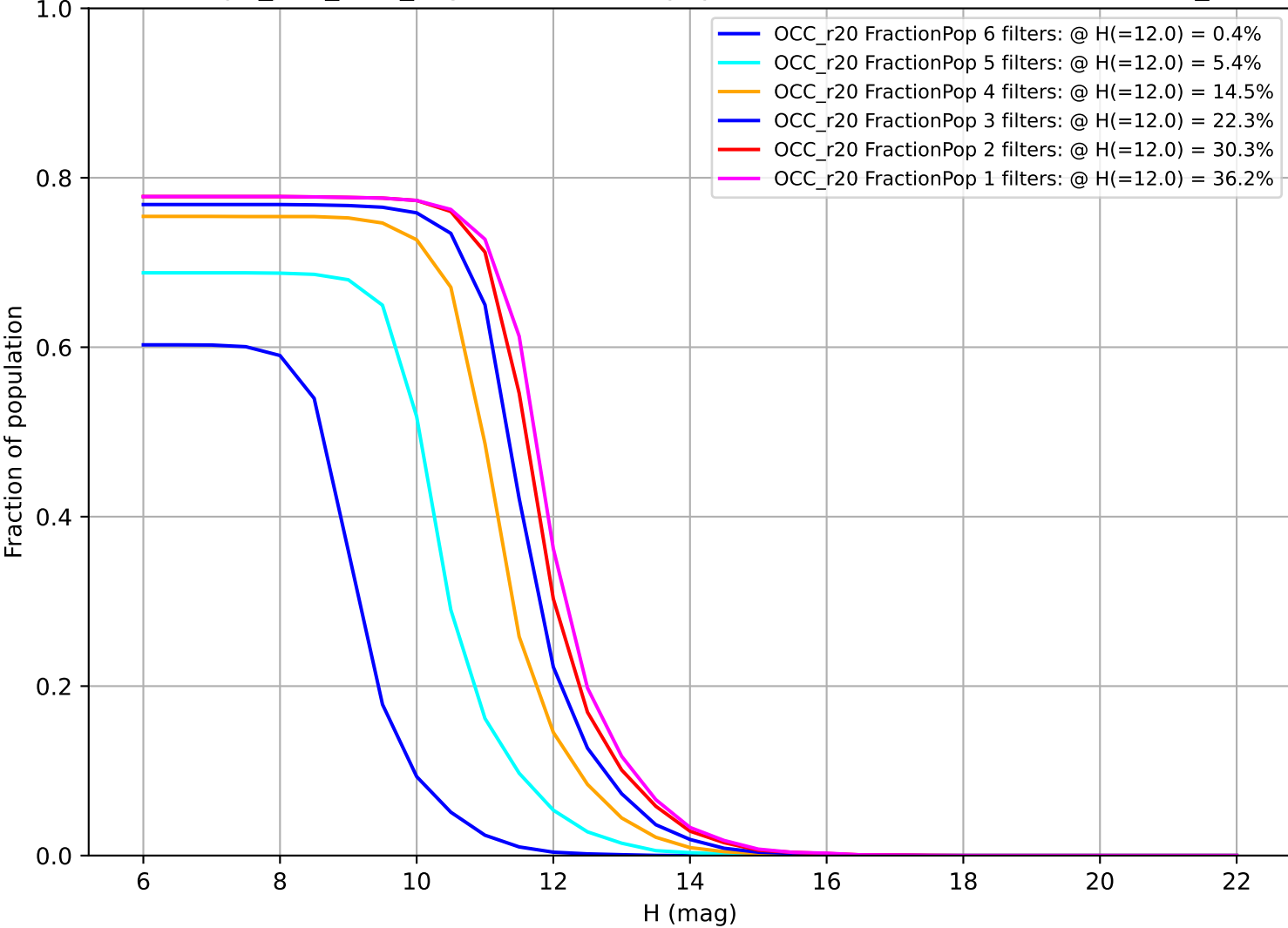
telescope_jerk_v3.5_10yrs: Fraction of population with colors in X filters OCC_r20
