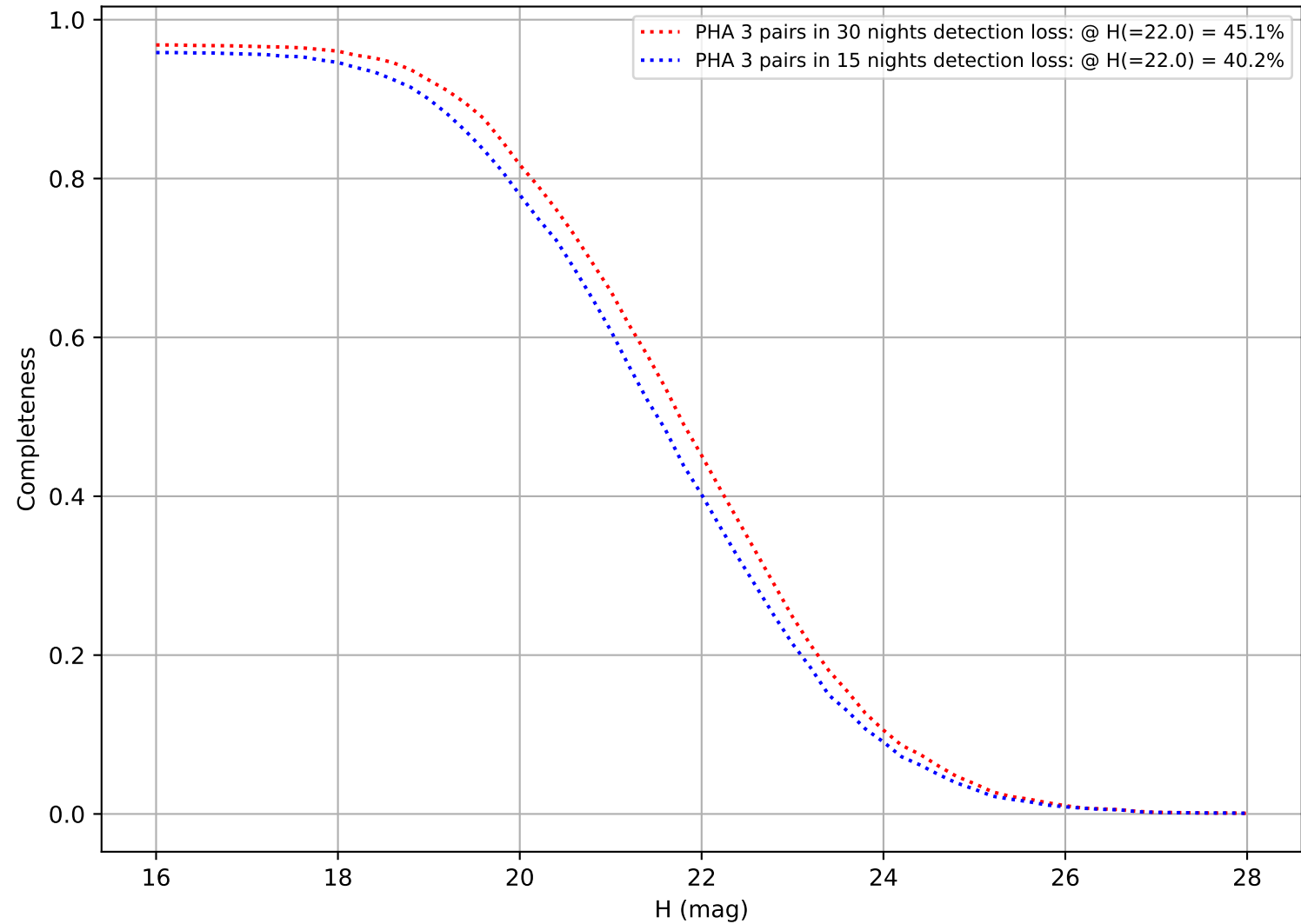
telescope_jerk_v3.5_10yrs: DifferentialCompleteness
