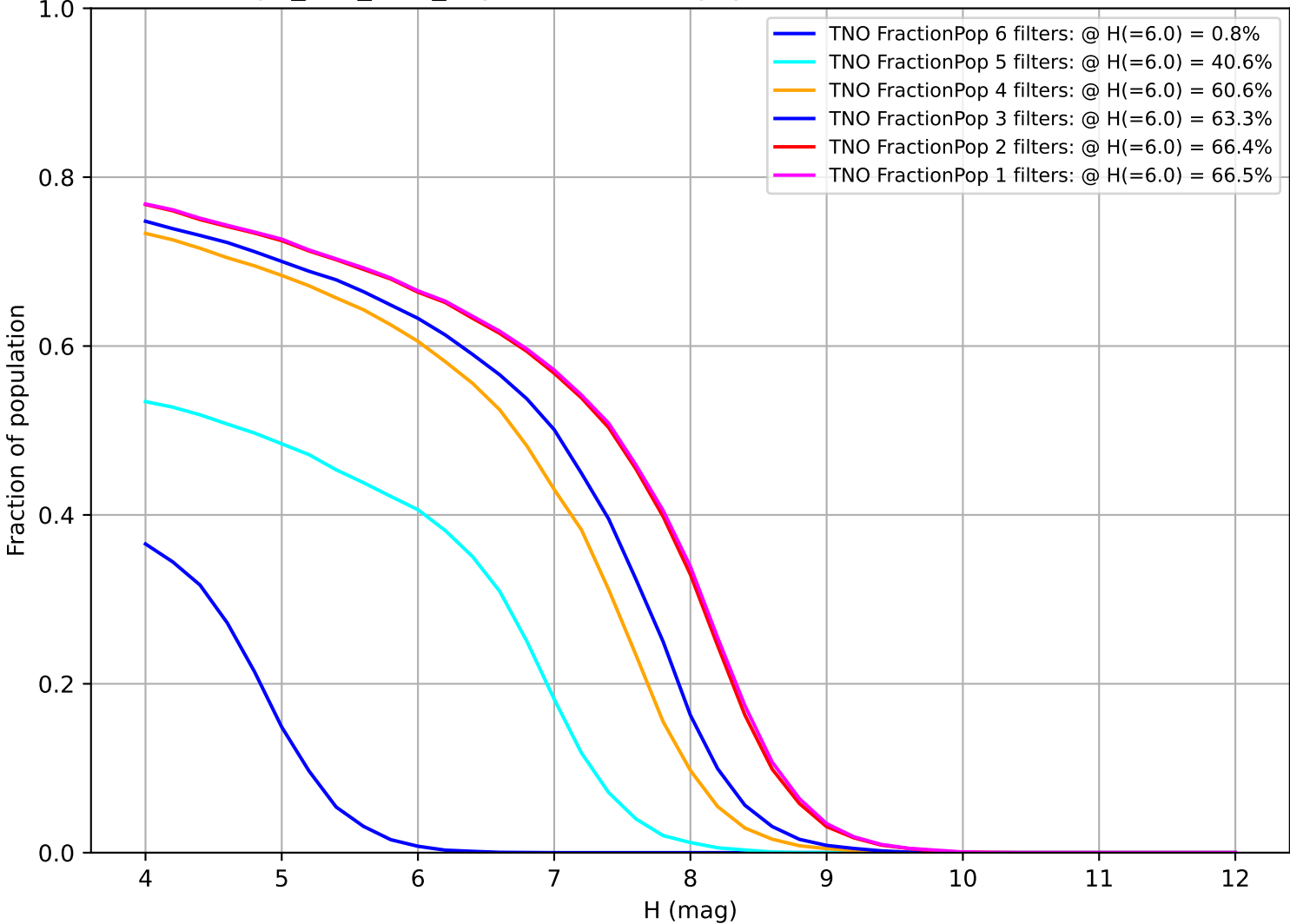
telescope_jerk_v3.5_10yrs: Fraction of population with colors in X filters TNO
