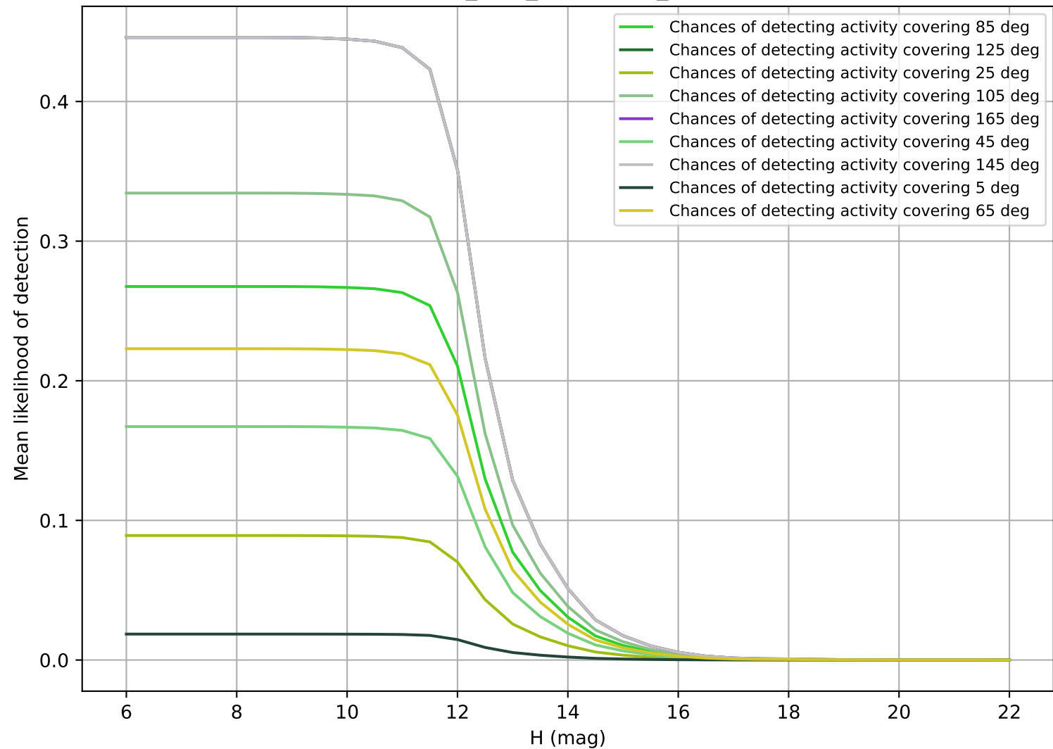
too_v3.5_10yrs OCC_r20
