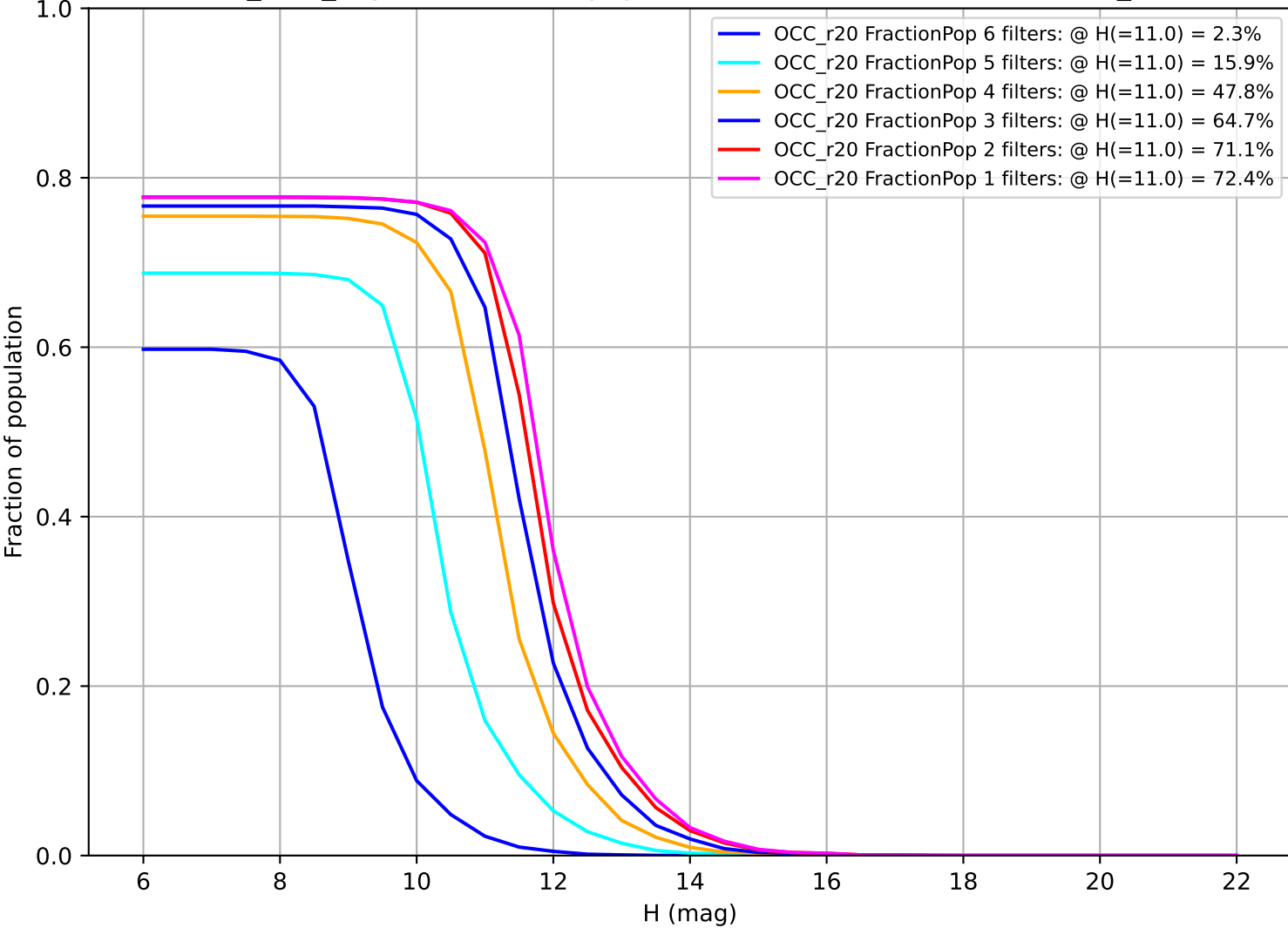
too_v3.5_10yrs: Fraction of population with colors in X filters OCC_r20
