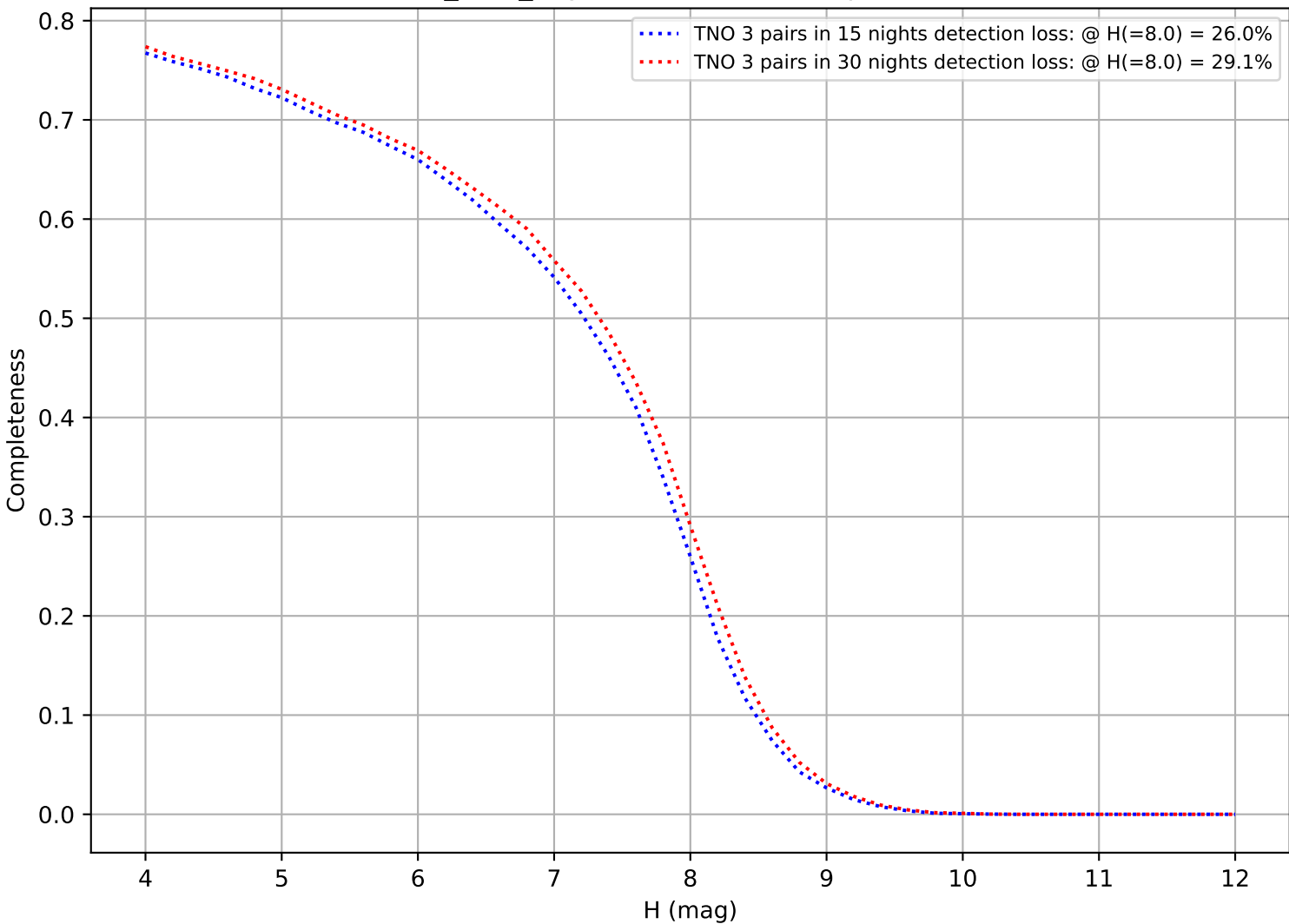
too_v3.5_10yrs: DifferentialCompleteness
