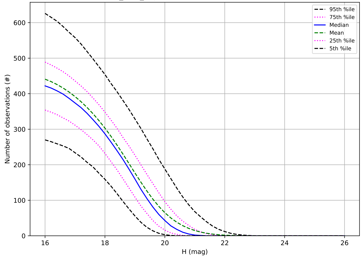
too_v3.5_10yrs: Number of observations MBA
