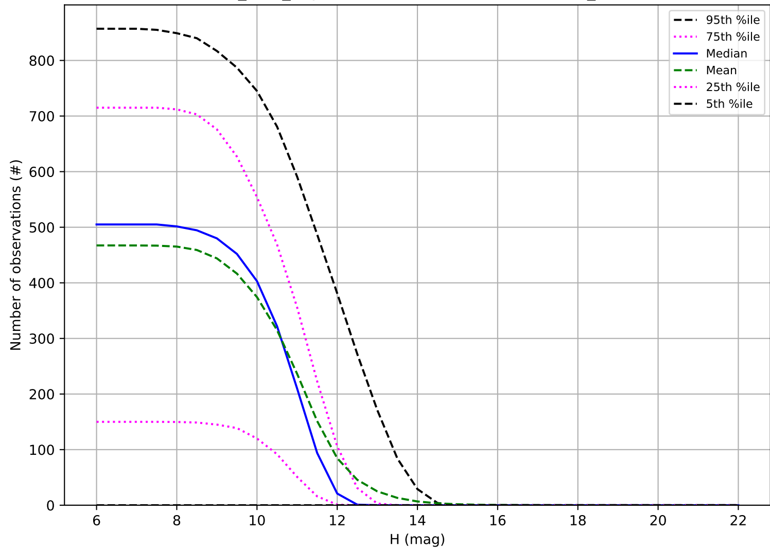
too_v3.5_10yrs: Number of observations OCC_r20
