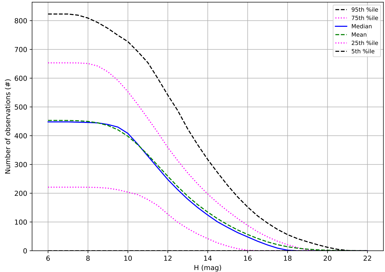
too_v3.5_10yrs: Number of observations OCC_r5
