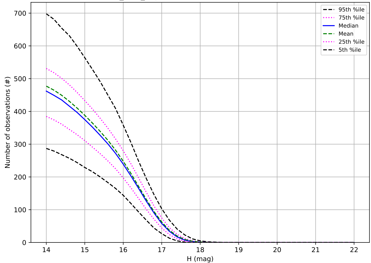
too_v3.5_10yrs: Number of observations Trojan
